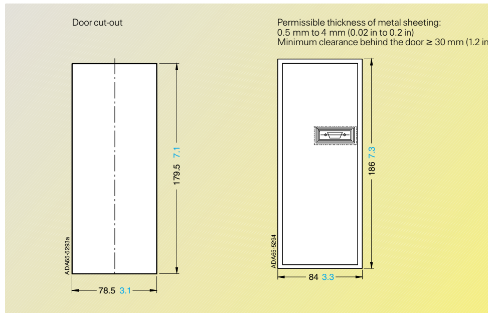
AOP1S/APMU adapter and door cut-out
