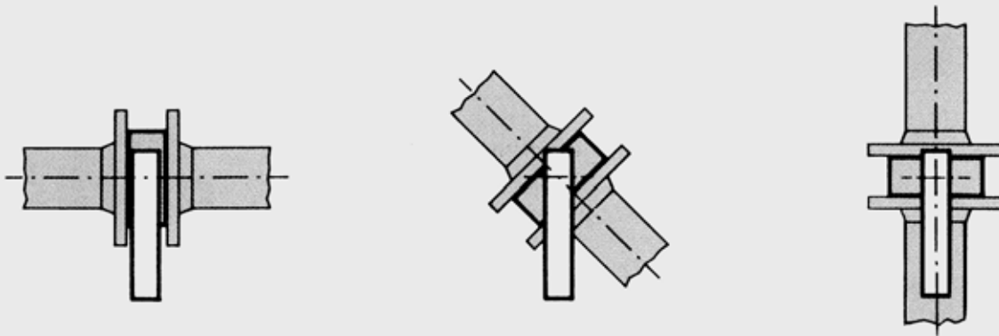
Fig. 3/98 Installation examples
