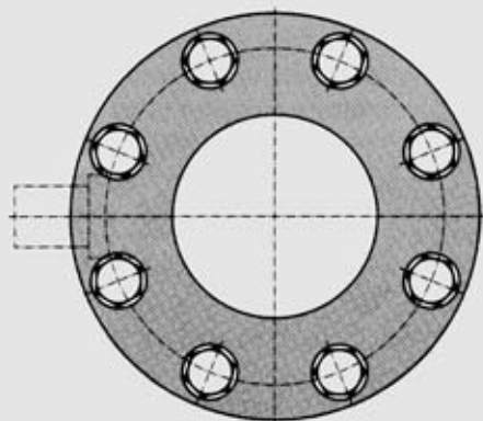
Fig. 3/99 Centering assembly
