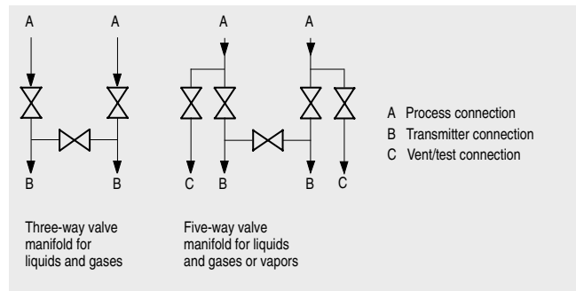
Fig. 1/87 Connections of the three-way and five-way valve manifolds
