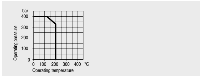
Fig. 1/88 Permissible operating pressure
