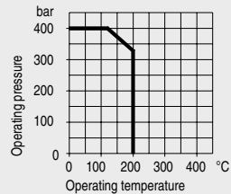
Fig. 1/92 Permissible operating pressure
