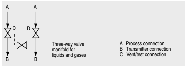
Fig. 1/91 Connections of the three-way valve manifold
