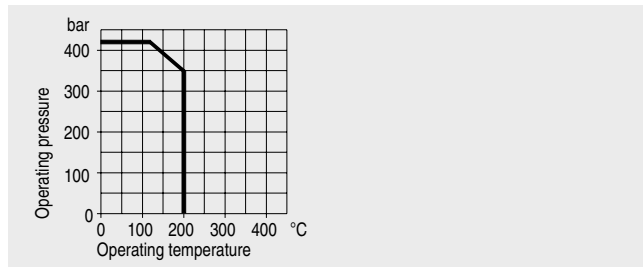
Fig. 1/103 Permissible operating pressure
