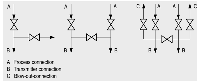
Fig. 1/102 Connections of the two-spindle, three-spindle and five-spindle valve manifolds
