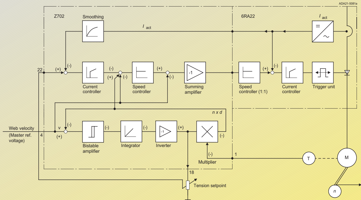
Fig. 1/18 Example: Simplified block diagram of an unwinder with indirect tension control
