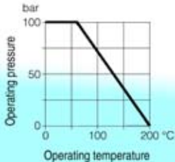
Fig. 1/76 Multiway cock PN 100 and permissible operating pressure as a function of the permissible operating temperature
